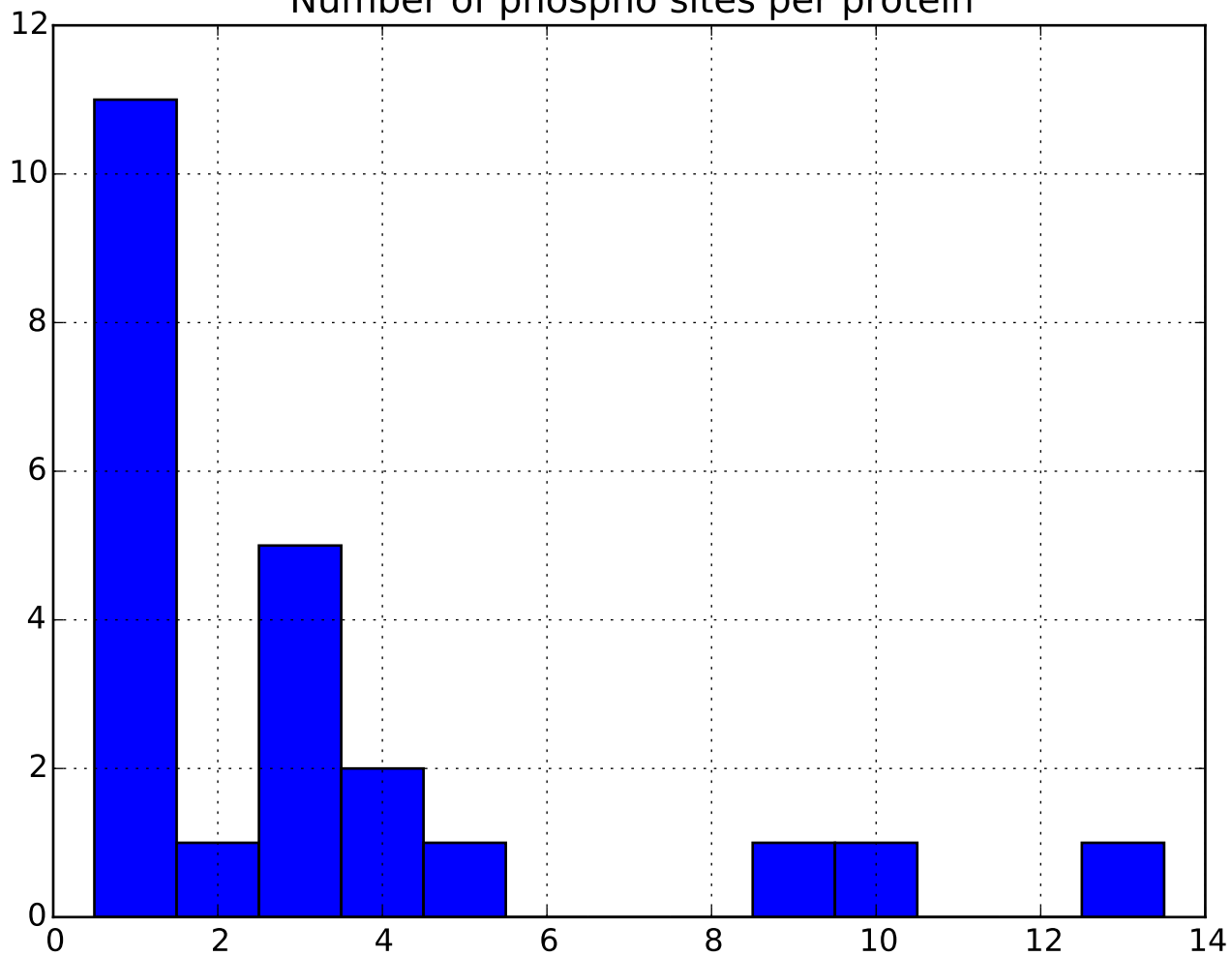
Number of phospho sites per protein
