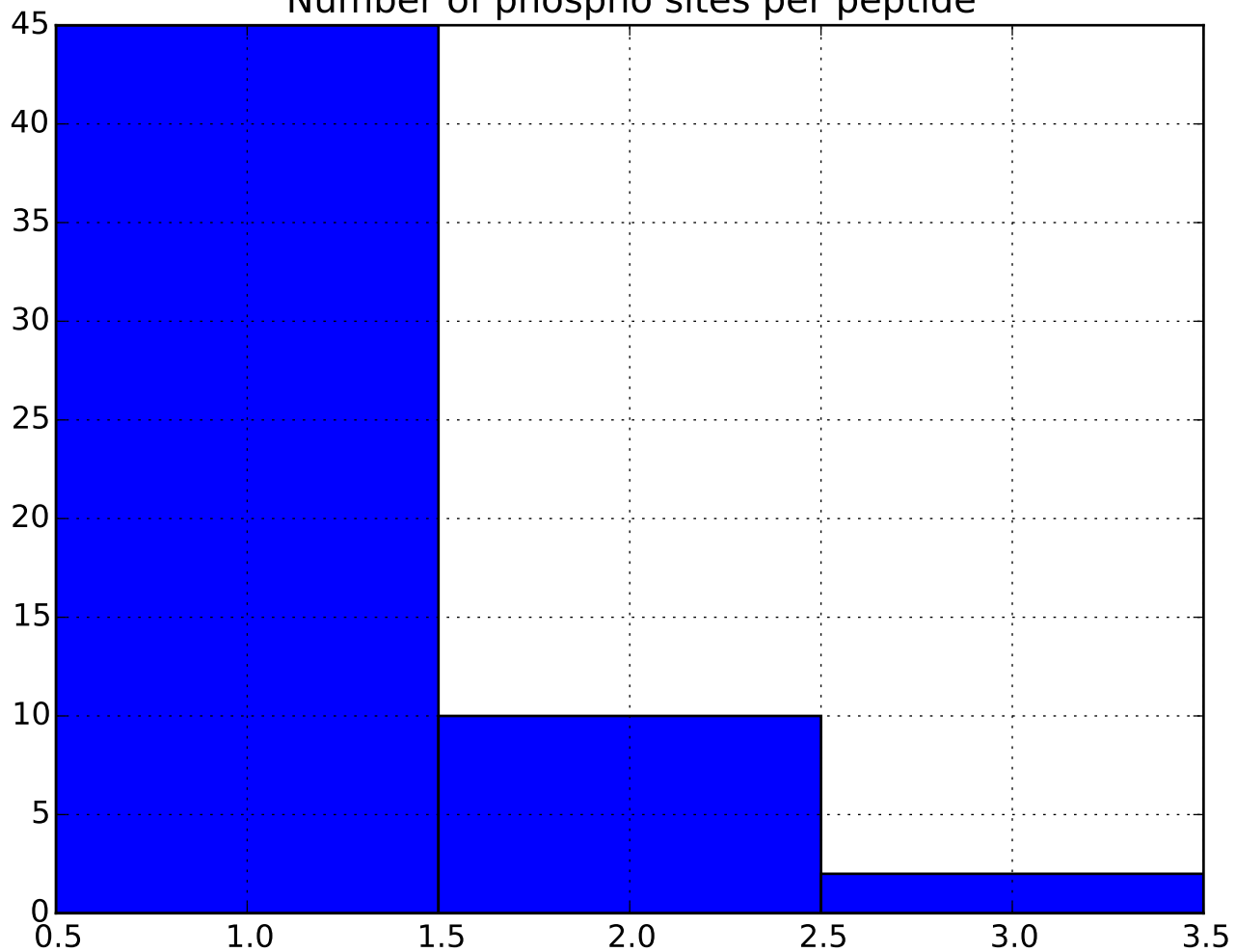
Number of phospho sites per peptide
