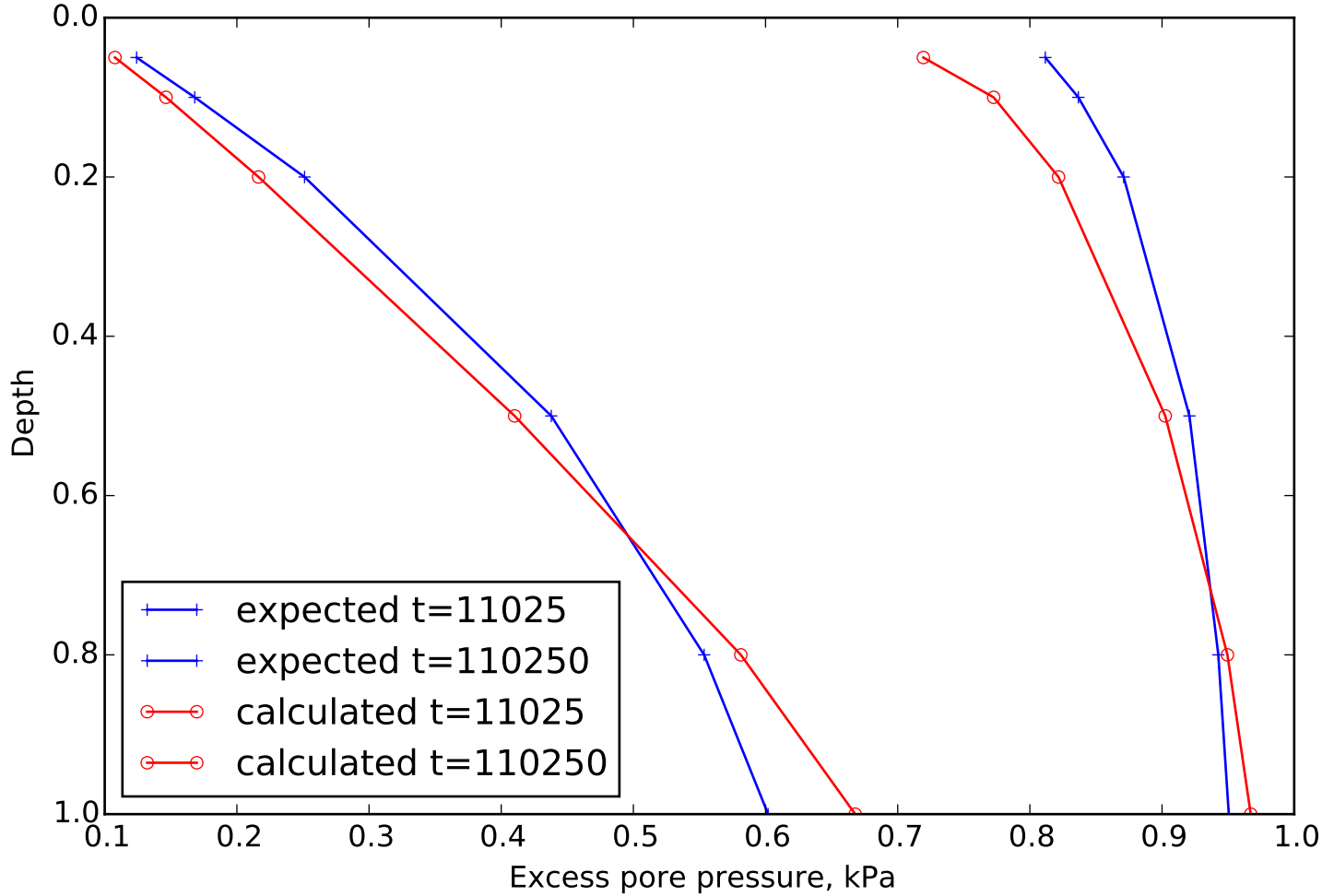
Deng et al. (2013) Radial drainage with linear depth dependent well resistance
