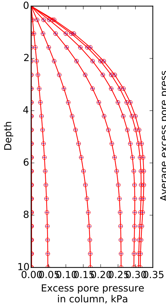
Lu et al (2010) Stone column, load is linear with depth
