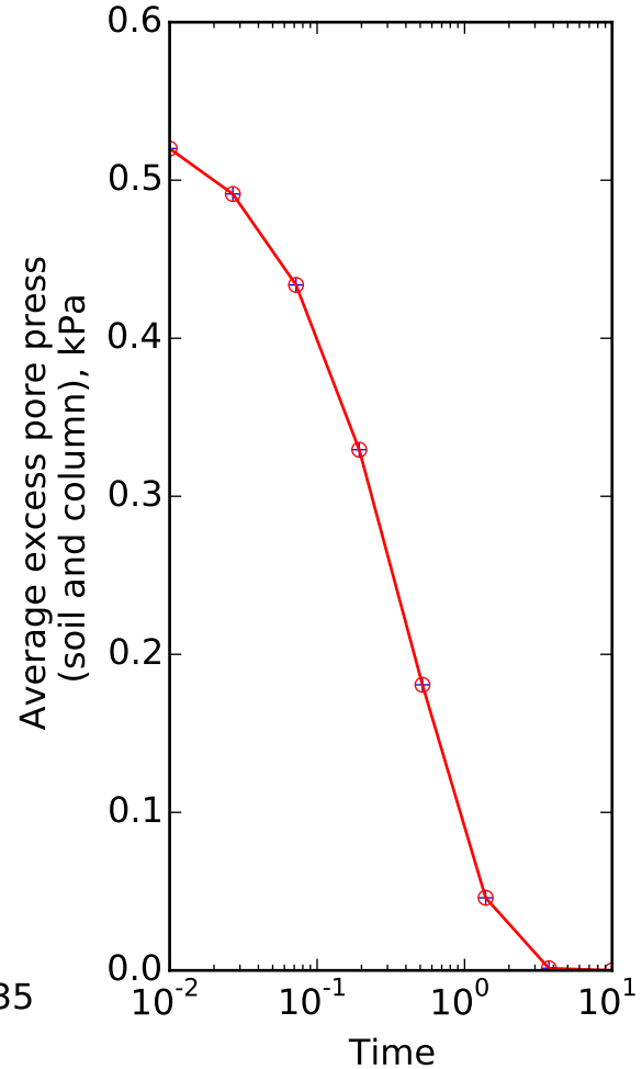
Lu et al (2010) Stone column, load is linear with depth
