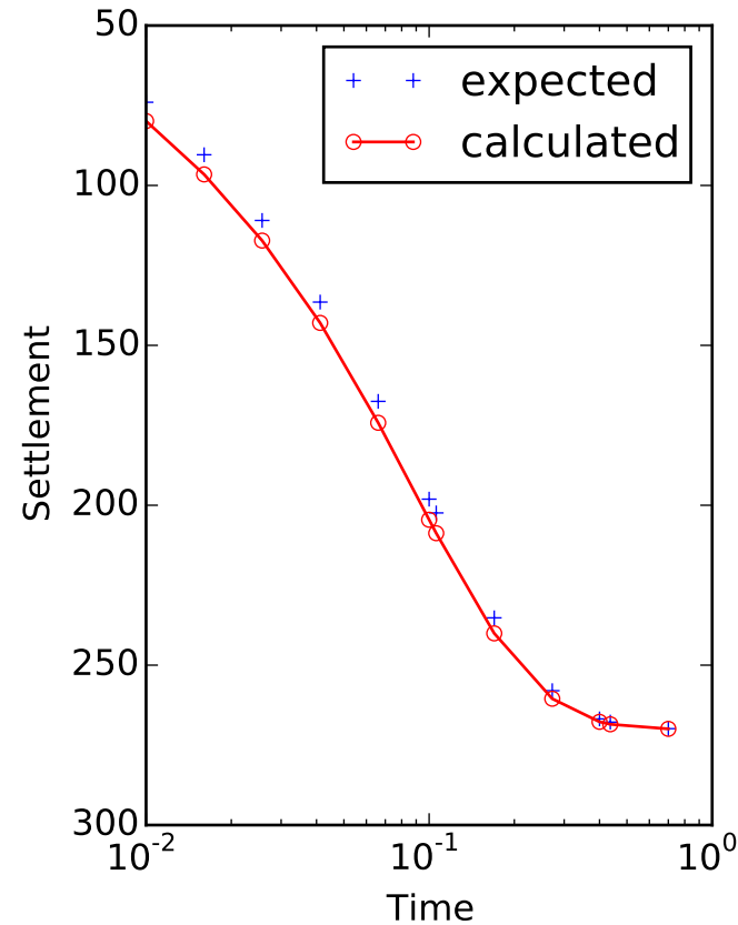
Nogami and li (2003) vertical and radial drainage free strain vs equal strain. Lambda=100
