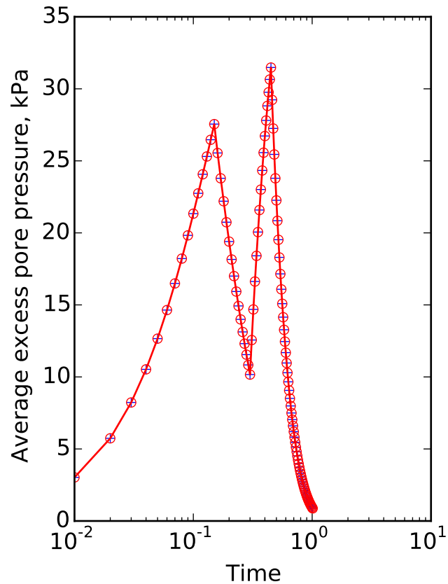
Tang and Onitsuka (2000) vertical and radial drainage
