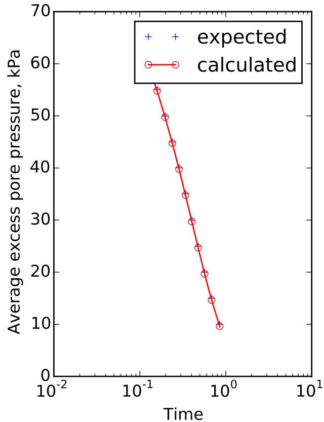
Mimic Terzaghi 1D by using time dependent pumping at mid-depth
