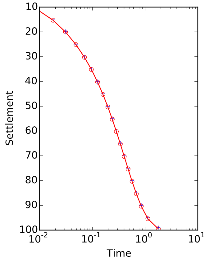
Mimic Terzaghi 1D by using time dependent bottom gradient boundary condition
