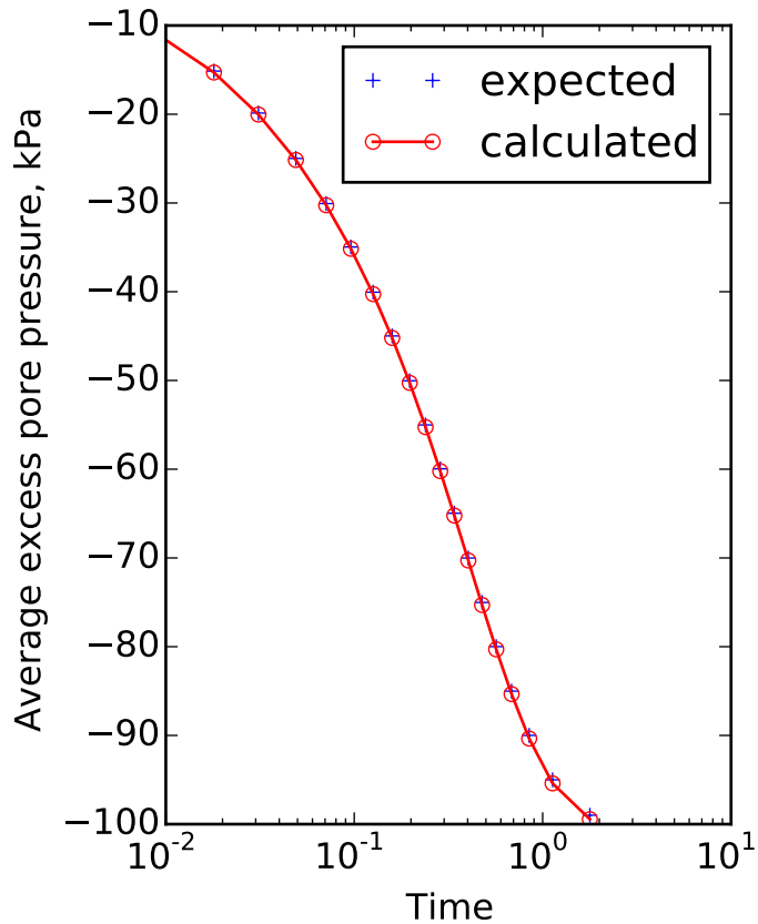
Mimic Terzaghi 1D by using time dependent bottom gradient boundary condition
