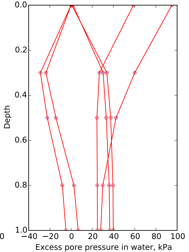
Shan et al. (2012) Unsaturated soil. instant surcharge + sinusoidal top water pressure boundary condition.
