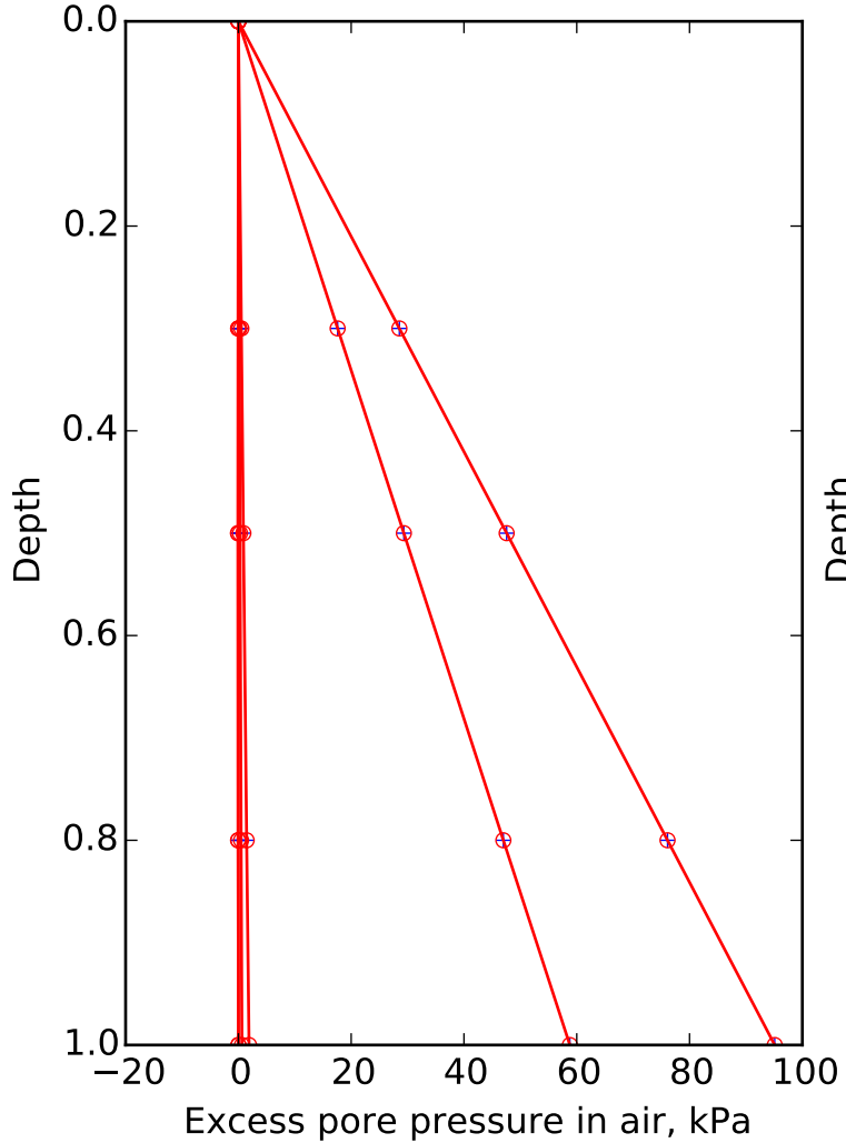
Shan et al. (2012) Unsaturated soil. instant surcharge + sinusoidal bot air pressure boundary condnsion.
