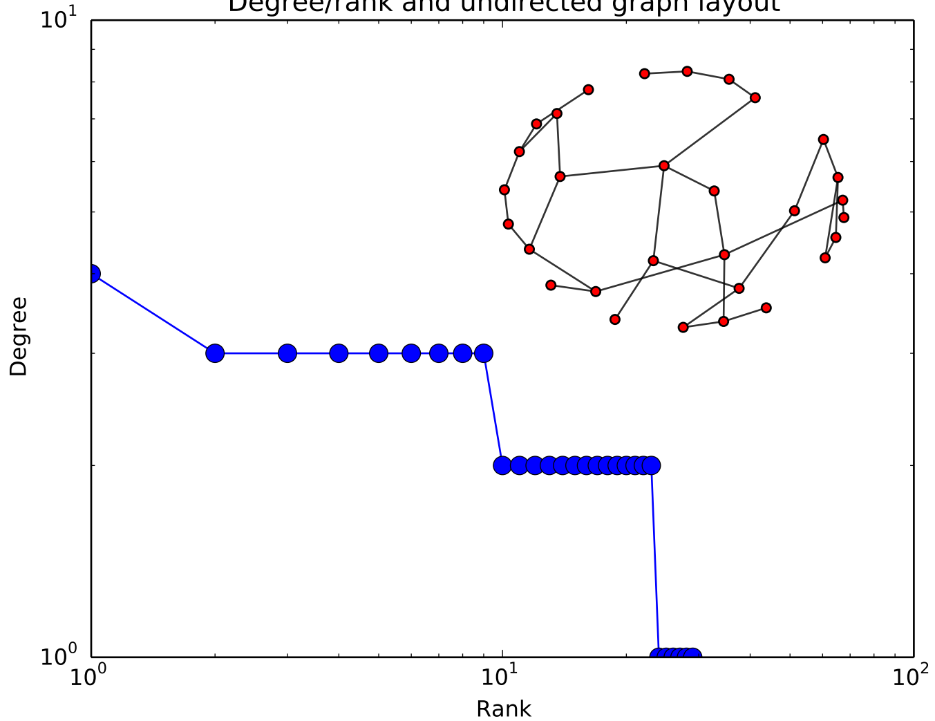
Degree/rank and undirected graph layout
