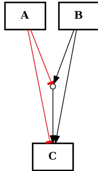
after call to expand_or_gates function
